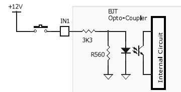
Input Circuit
