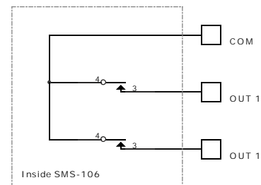
Output Circuit
