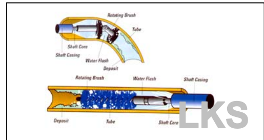
Wheel Brush Assembly for Curved Tube I.D. P/N : S-PE-WBC-XXX
